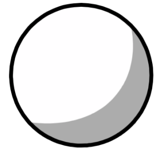
sphere
