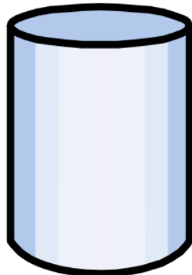
cylinder
