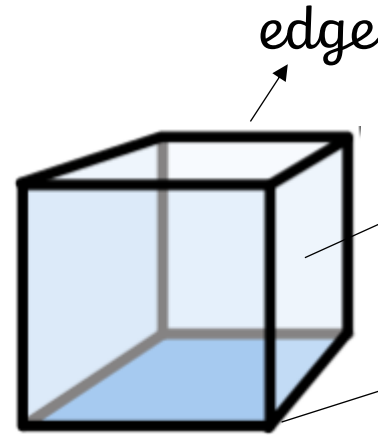
cube
