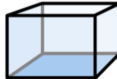
cuboid
